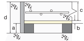
Fig 7.2 a) Isomat Isolators: 50mm b) Plywood: 15mm c) Concrete slab: 100mm d) Overall height: 165mm
