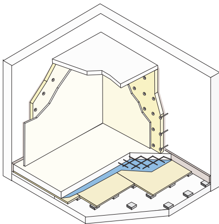
Fig 2.2 Recording Studios, Nightclubs, Plant Rooms etc. Internal walls and structures can be installed onto the floating slab to create a box in box structure with the acoustic air void created on all sides.
