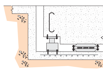
Fig 8.1 FSL spring and FV damper low frequency isolated foundation.
