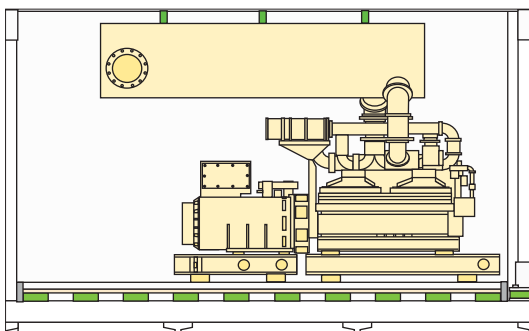
Fig 2.3 Plant rooms
