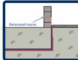
Verlimber VR27 used as raft-slab isolation
