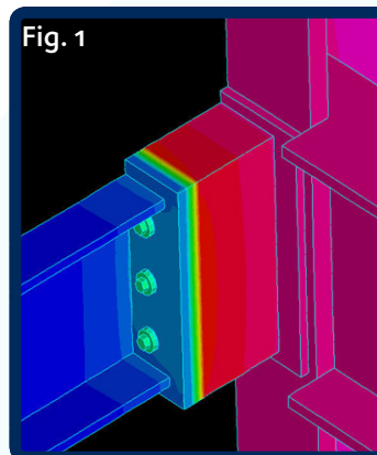
Fig. 1 shows the predicted temperature distribution with a Farrat TBL Structural Thermal Break Plate and Thermal Isolating Washers. The temperature on the steelwork on the warm side of the cladding system is increased to 16.5°C and the heat loss (X-value) is reduced to 0.35 W/K, a 73% decrease in the heat loss.
